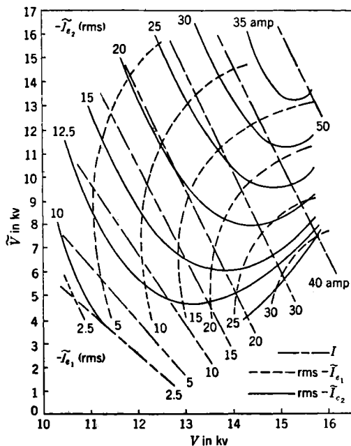
Fig. 7-27.—Plots of d-c current \bar{I} and a-c currents \bar{I}_{e_1} and \bar{I}_{e_2} in the \tilde{V} - V -plane.
